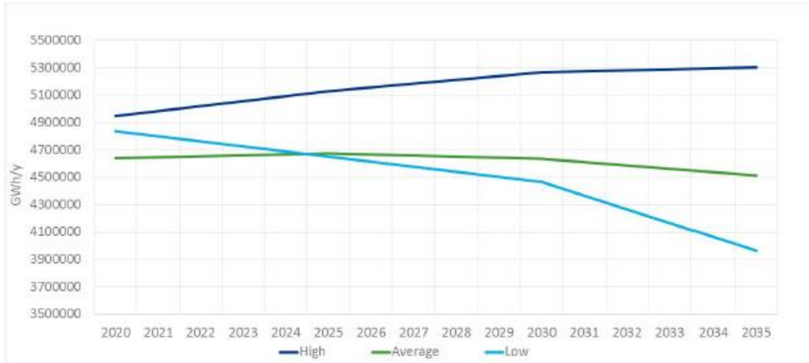
Gas demand scenarios of the FROG study
